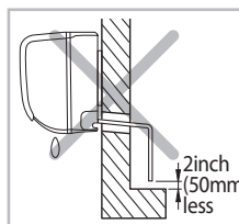
Keep a clearance of at least 2inch(50mm) between the end of the drain hose and the ground.
