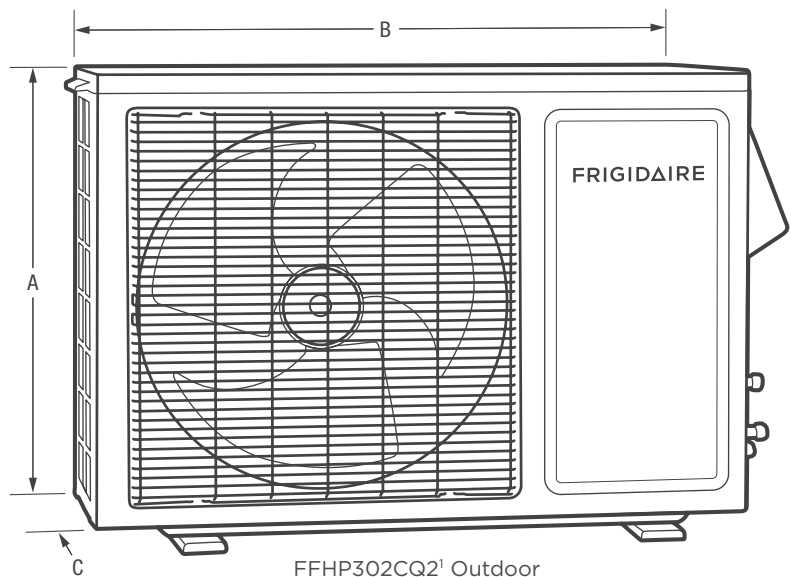
FFHP302CQ2 1 Outdoor
