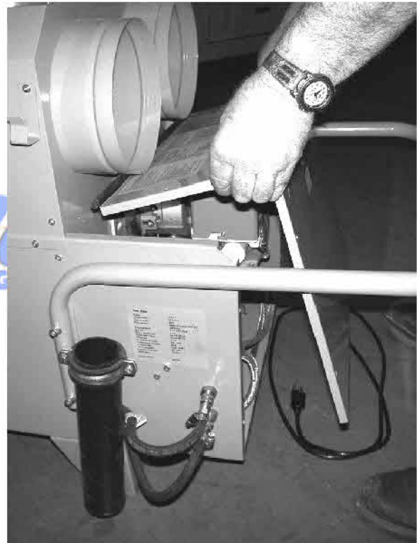
Remove the fuel pump/blower assembly housing and guard plate
