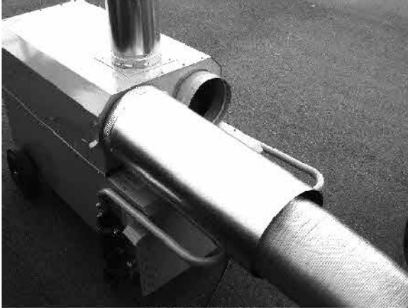
Slide the heat shields in place
