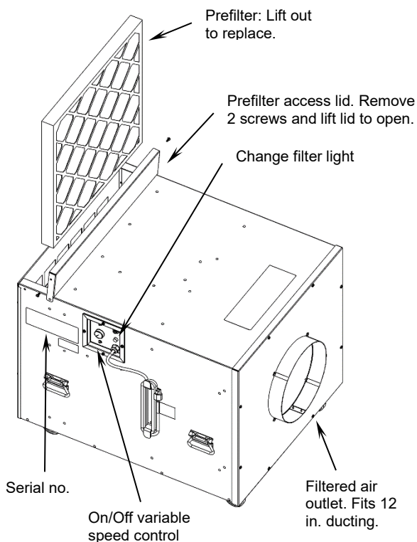
Fig 1: Changing the Prefilter
