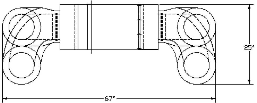
CONDENSER DUCTING
