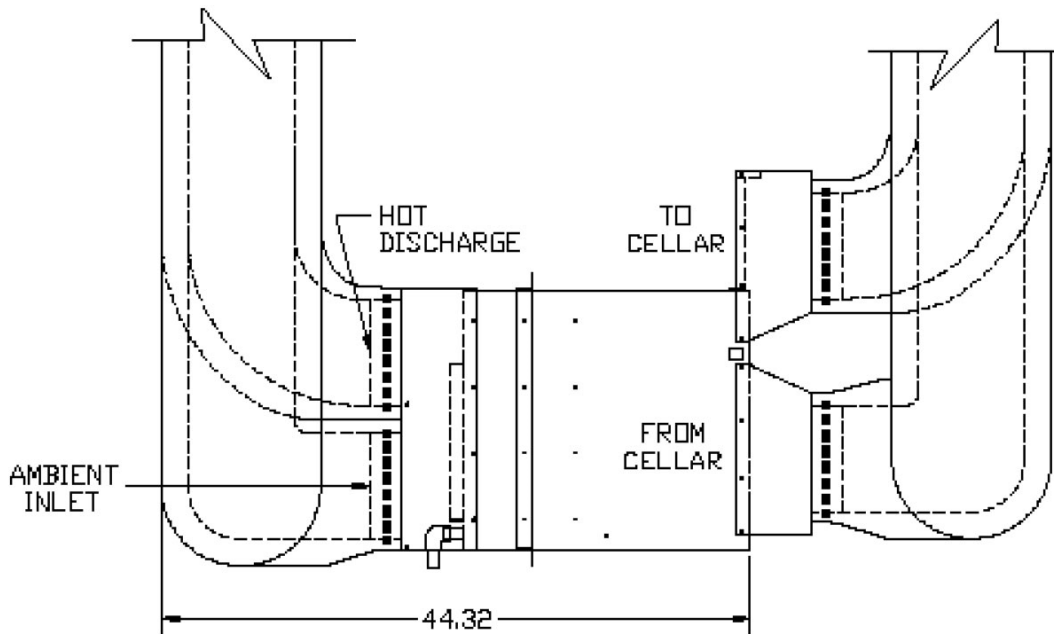
CONDENSER DUCTING
